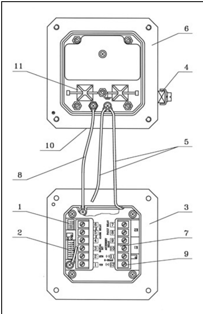
Figure 5. UV Flame Detector with Cover Removed
