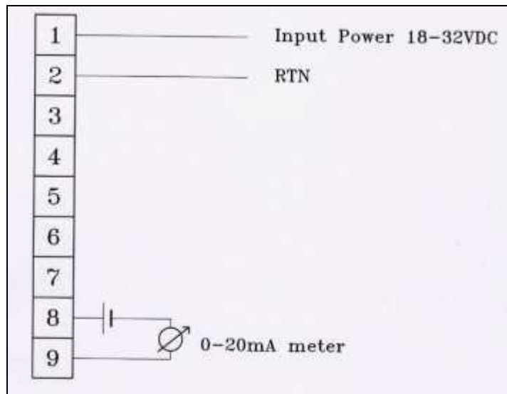
Figure 9: 0-20mA Wiring (Sink) 4-Wire Connection
