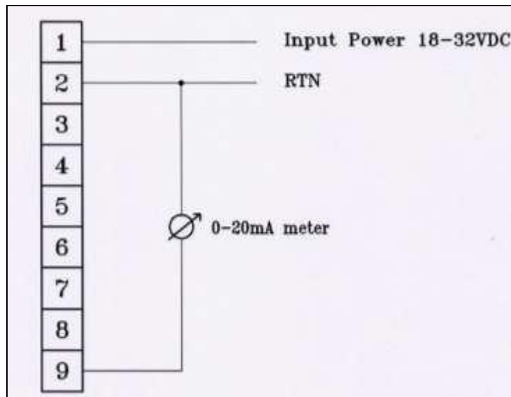
Figure 10: 0-20mA Wiring (Source) 3-Wire Connection
