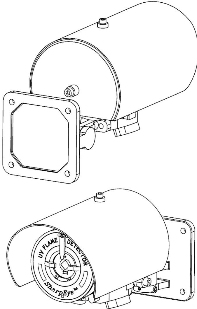
Figure 16: Weather Protection
