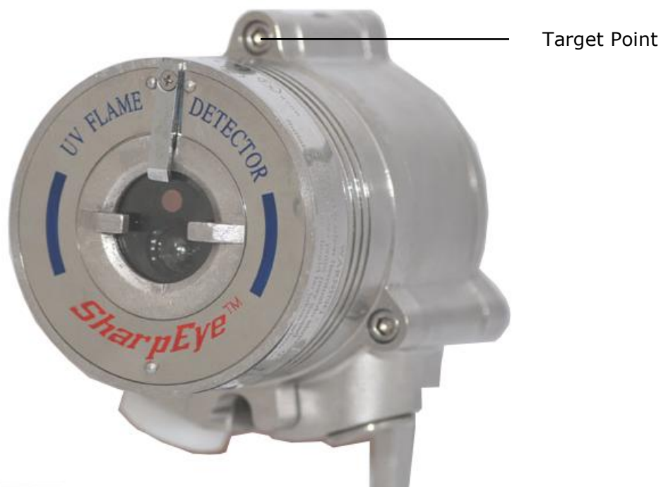
Figure 14: 40/40U and UB Detector Target Point
