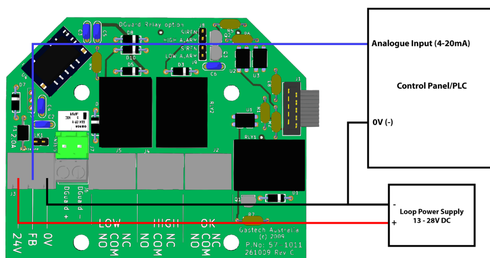
Figure 31. D-Guard 2 R Electrical connections.
