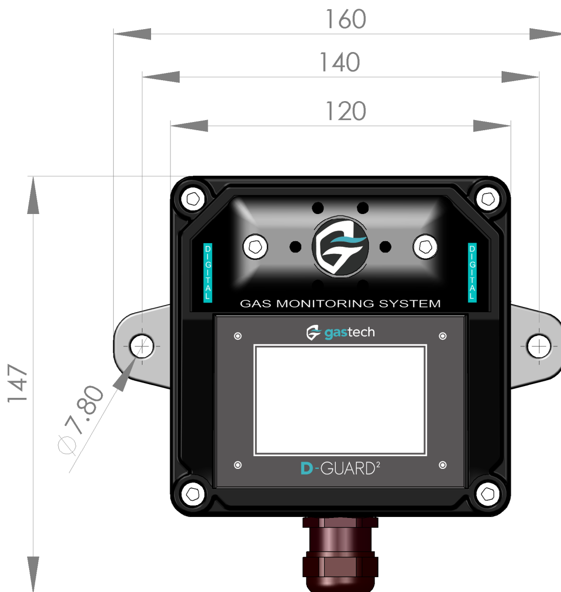
Figure 26. D-Guard 2 R dimensions in millimetres (front view).
