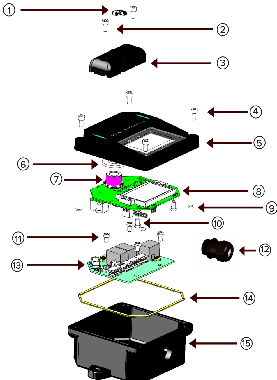
Figure 34. D-Guard 2 R replacement parts - exploded view.
