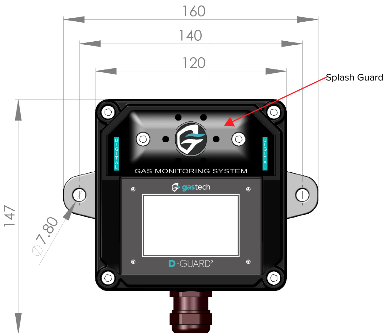
Figure 4. D-Guard 2 R mounting dimensions in millimetres.
