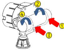
Horizontal Mounted
