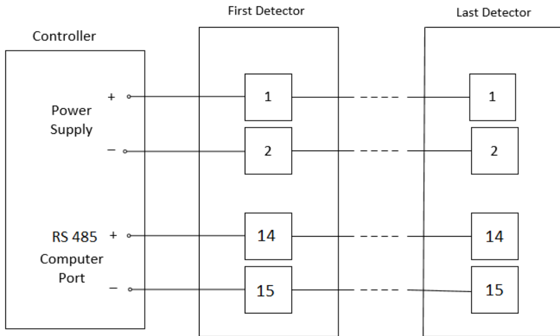
Figure 20: RS-485 Networking
