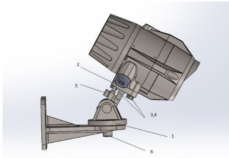
FIGURE 13 - DETECTOR ON TILT MOUNT – SIDE VIEW
