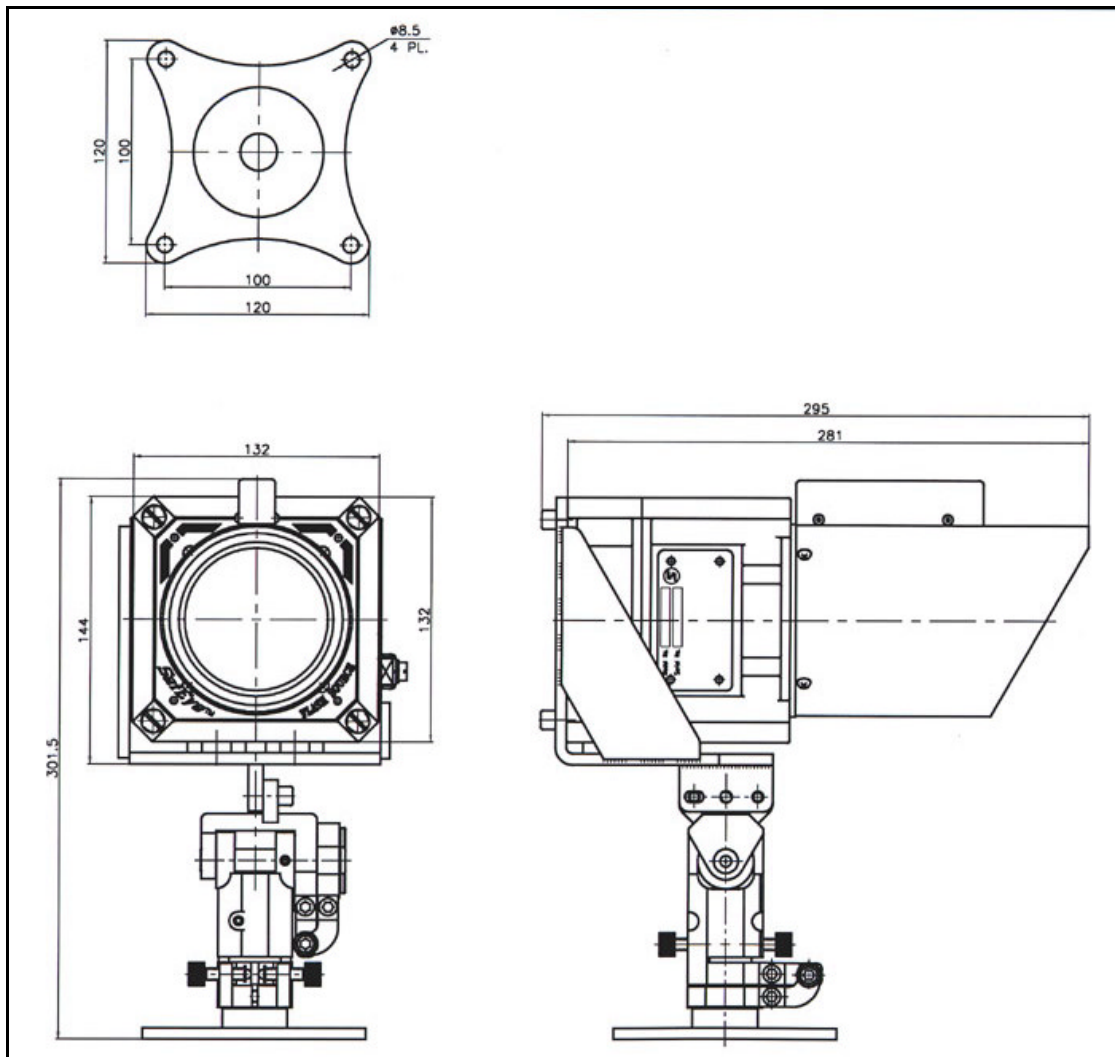
Figure 27. Source and Tilt Mount Outline Drawing
