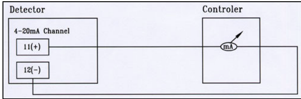
Figure 19. 4-20mA Source Output
