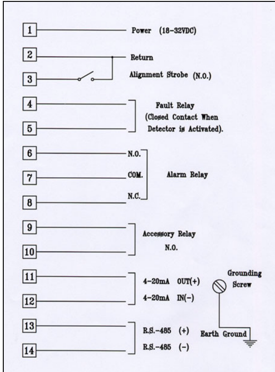
Figure 18. Detector's Wiring Diagram
