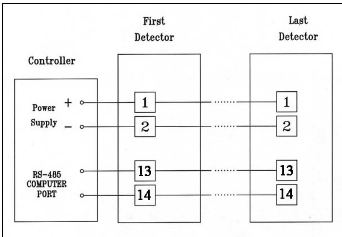
Figure 21. RS-485 Networking
