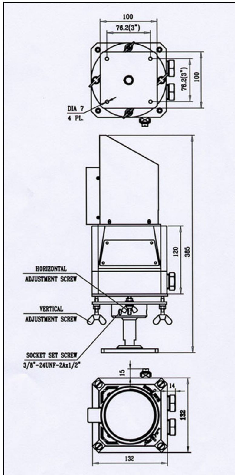
Figure 24. Source Outline Drawing (80 dia Lens Type) With Swivel Mount
