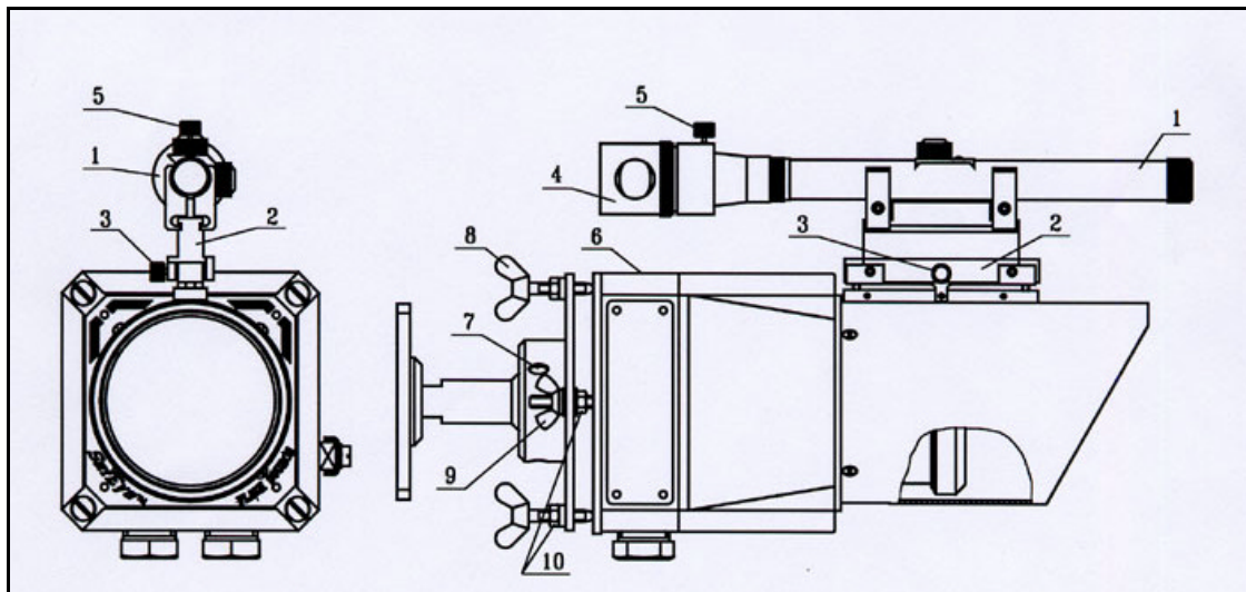
Figure 16. Alignment and Mode Selection
