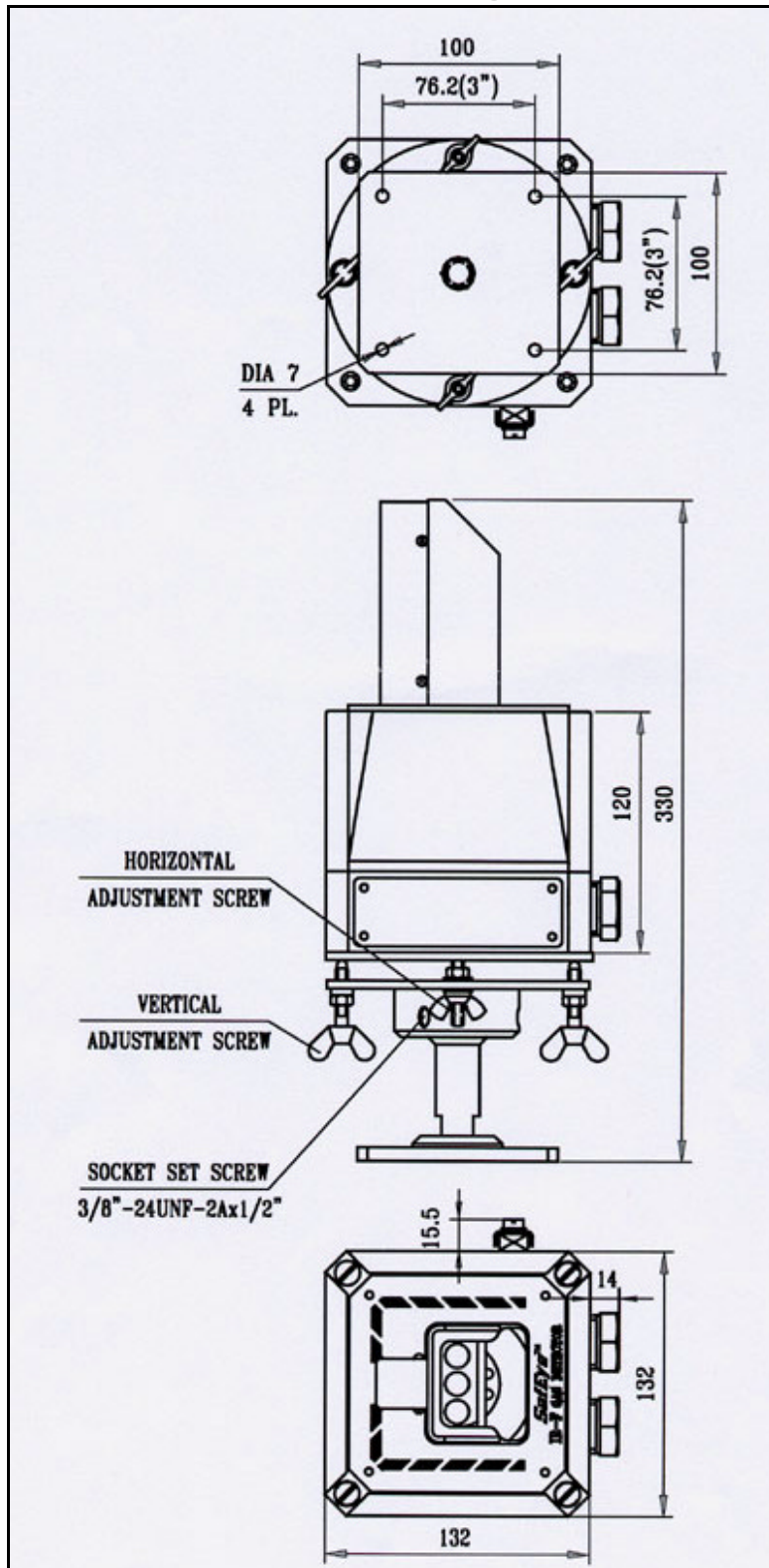
Figure 22. Detector Outline Drawing With Swivel Mount
