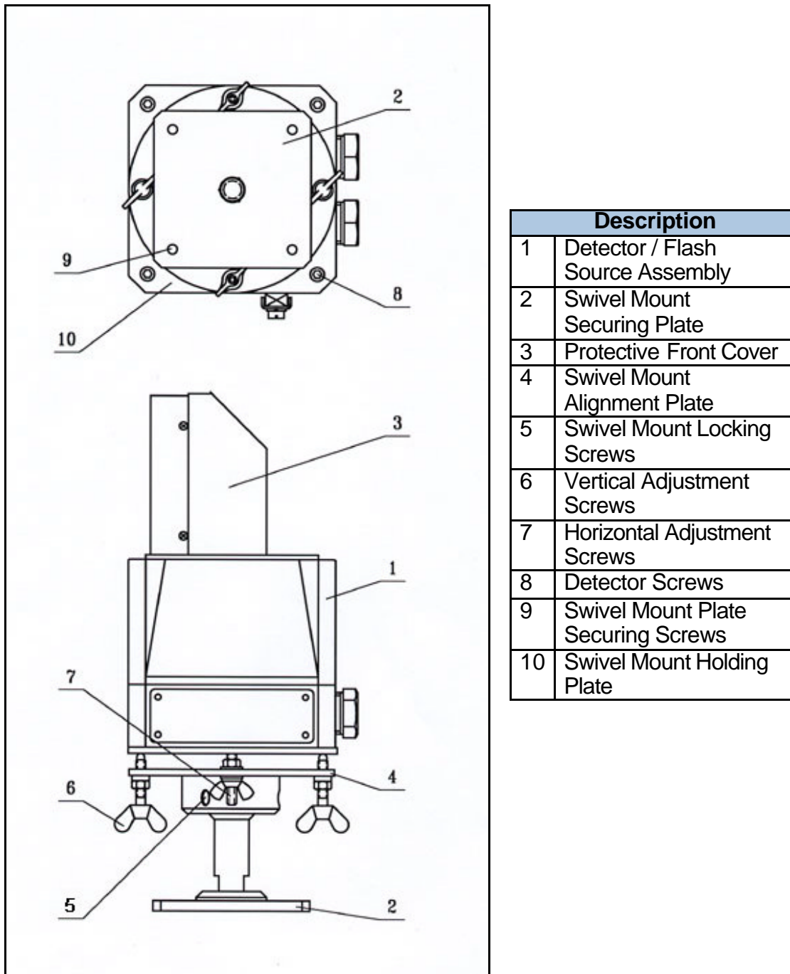
Figure 7. Detector/Flash Source and Swivel Mount Assembly for Standard Installation
