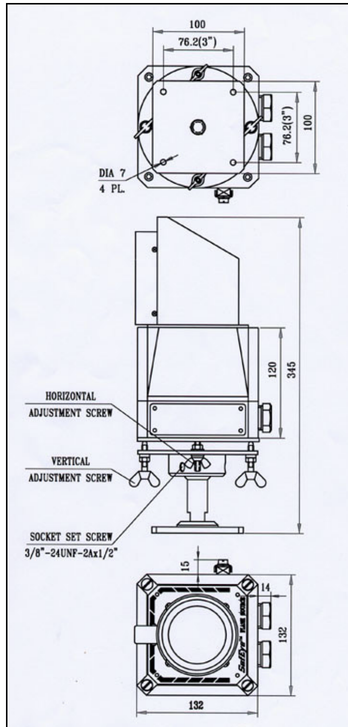
Figure 23. Source Outline Drawing (65 dia Lens Type) With Swivel Mount
