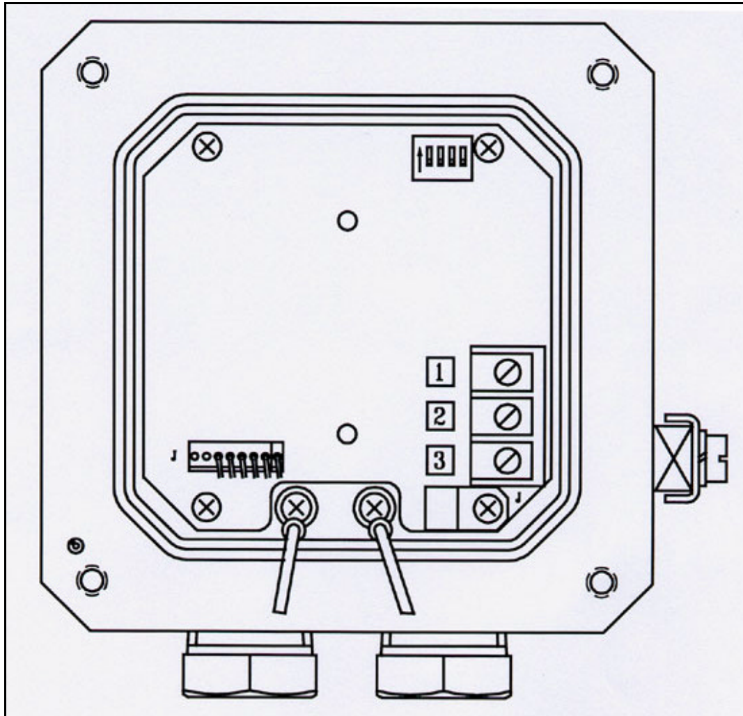
Figure 6. Flash Source Terminal Board
