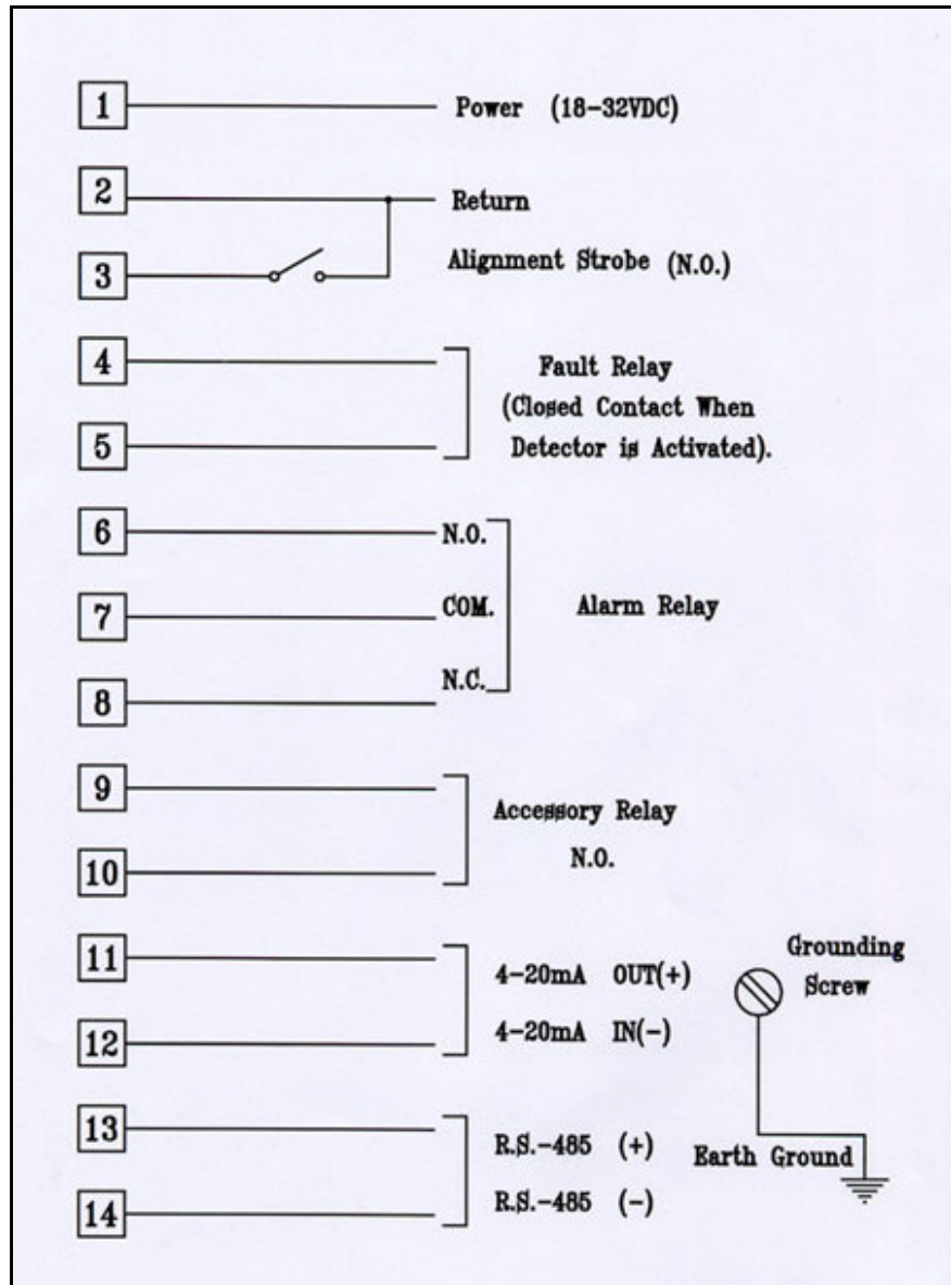
Figure 4. Detector's Wiring Diagram
