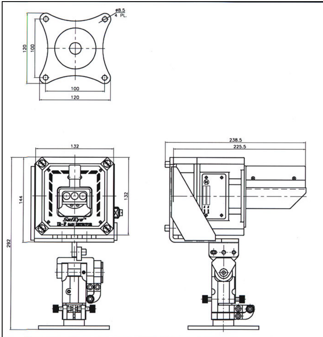
Figure 26. Detector and Tilt Mount Outline Drawing
