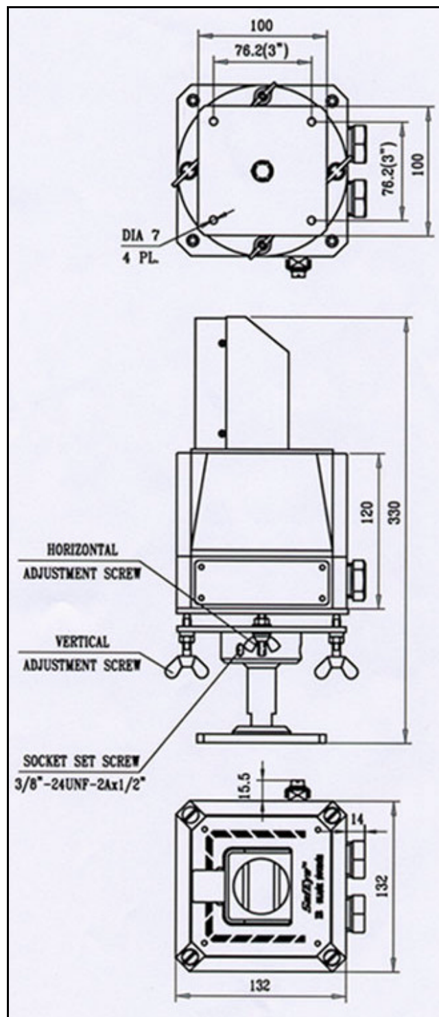
Figure 25. Source Outline Drawing (Reflector Type) With Swivel Mount
