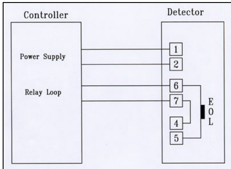
Figure 20. Typical 4 Wire Controller
