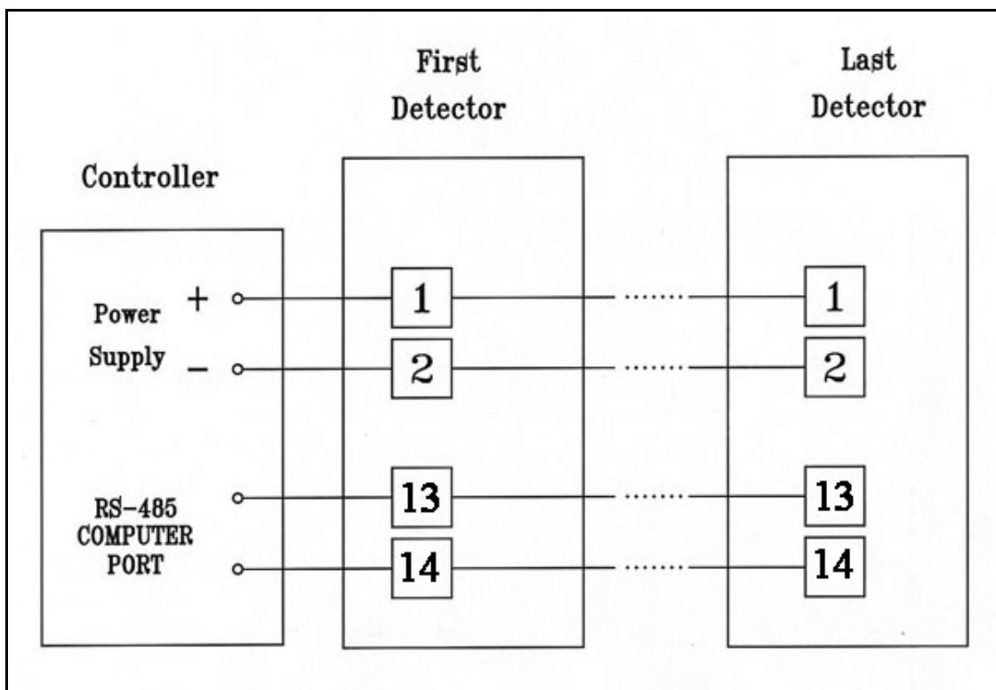
Figure 20. RS-485 Networking
