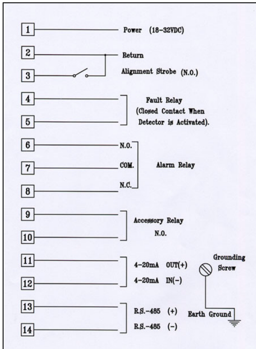
Figure 3. Detector's Wiring Diagram
