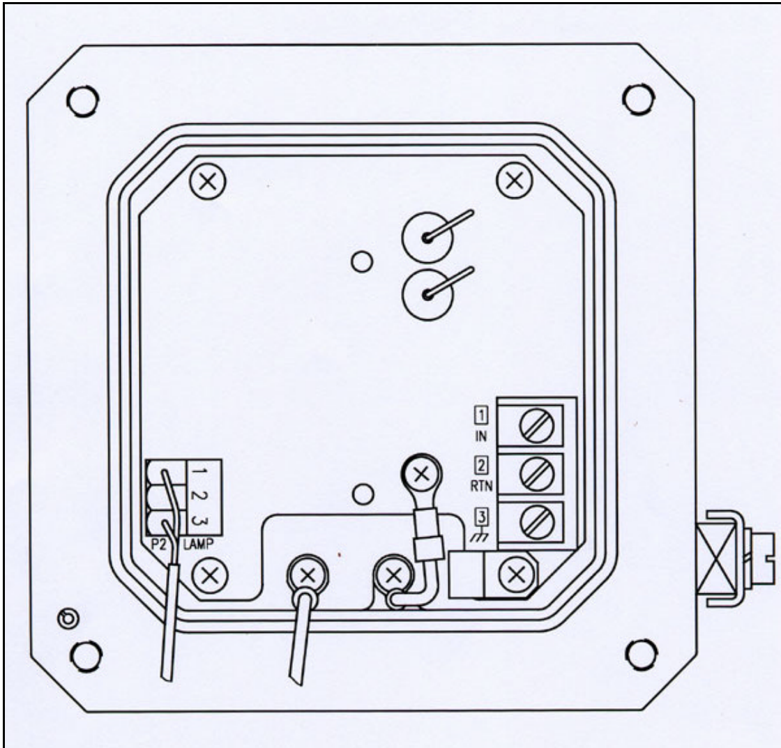
Figure 5. Light Source Terminal Board
