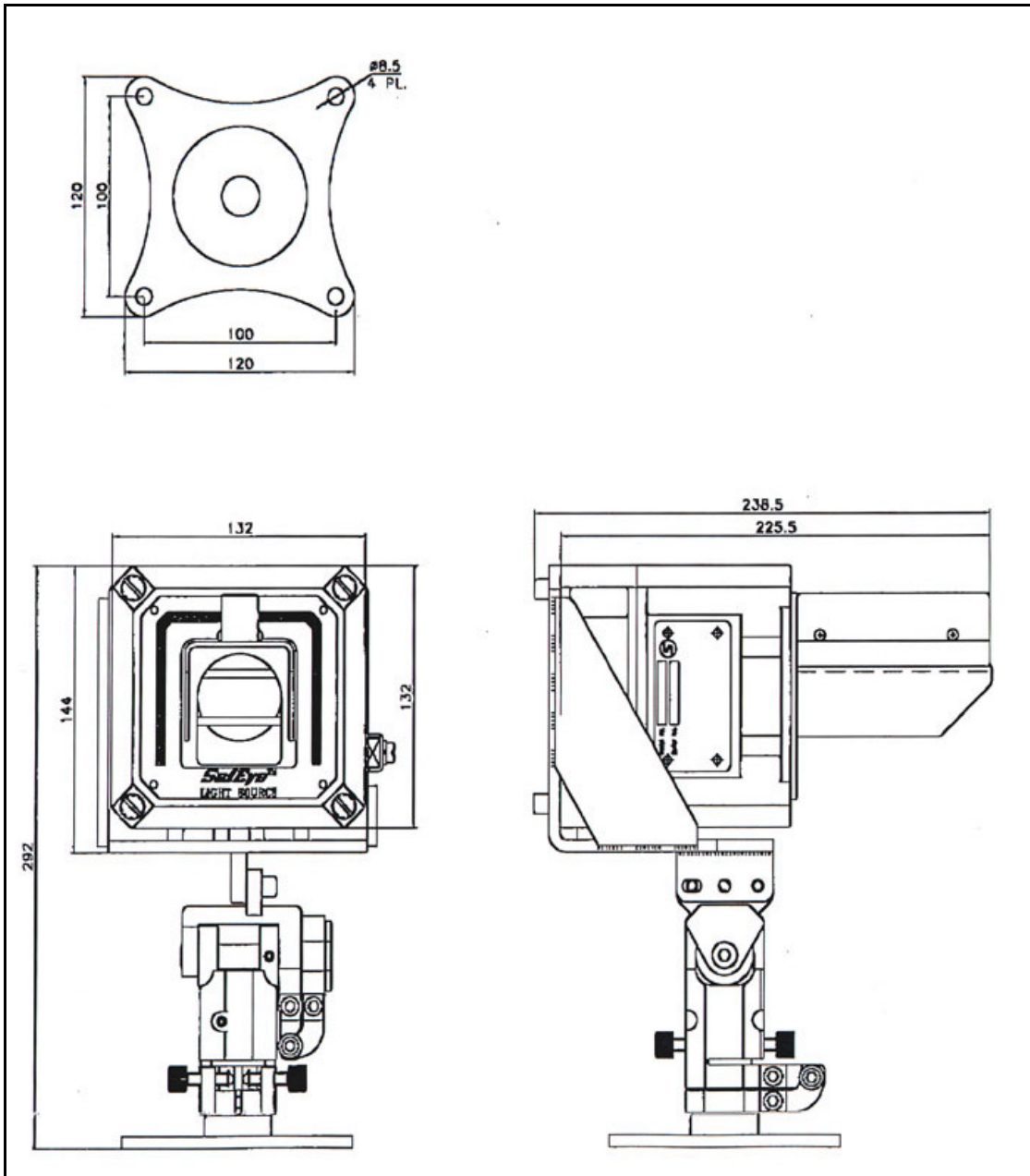
Figure 24. Source and Tilt Mount Outline Drawing
