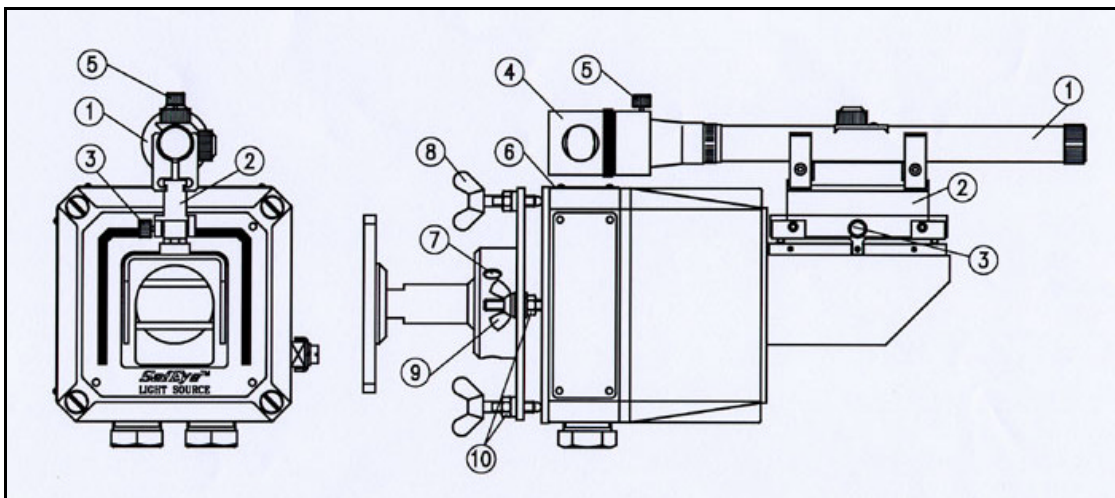
Figure 15. Alignment and Mode Selection
