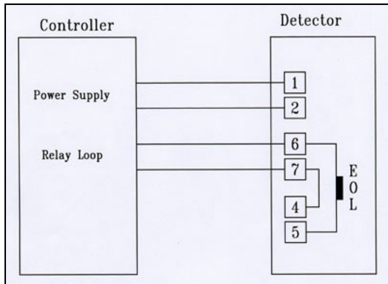
Figure 19. Typical 4 Wire Controller
