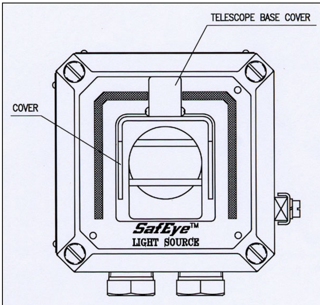
Figure 1: Light Source – Reflector Type
