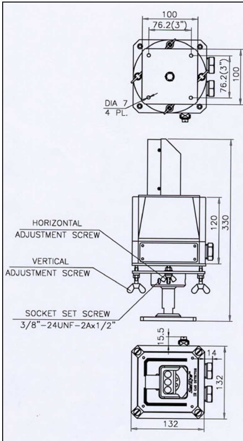
Figure 21. Detector Outline Drawing With Swivel Mount
