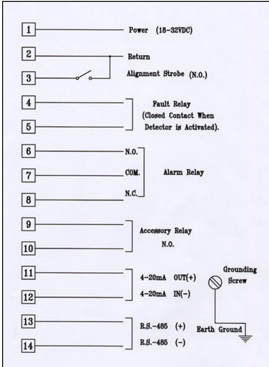
Figure 17. Detector's Wiring Diagram
