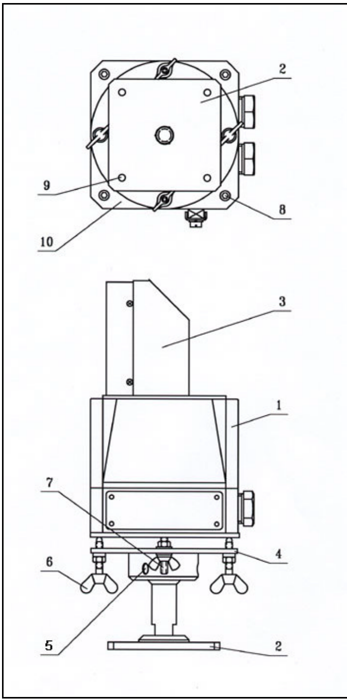
Figure 6. Detector/Light Source and Swivel Mount Assembly for Standard Installation
