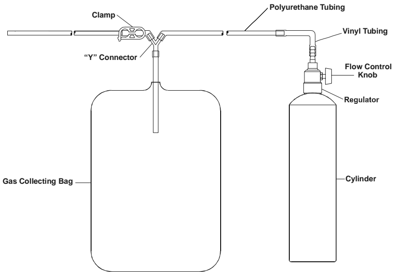
Figure 4-1 Calibration Kit with Gas Cylinder and Gas Collecting Bag
