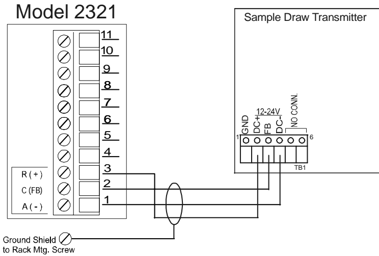
Figure B-4 Model 2321 External Wiring
